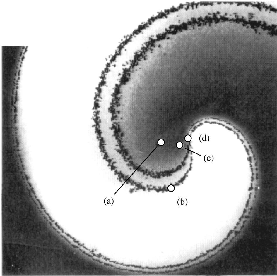
Figure 4.1: A spiral wave pattern in the Belousov-Zhabotinsky reaction; courtesy of [MZ94].
