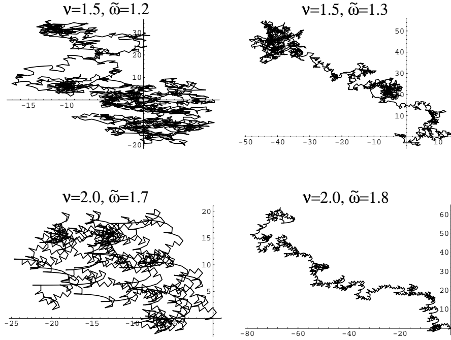
Figure 8.1: Sample paths of Brownian tip motions.
