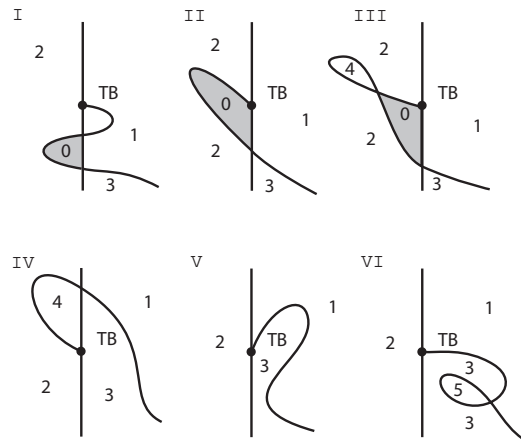
Figure 1. Qualitative bifurcation diagrams I – VI in the (b_0, b_1) -plane. Vertical b_1 -axis at b_0 = -a coincides with zero eigenvalues \eta . Takens-Bogdanov point TB, emanating Hopf bifurcation curve, and resulting unstable dimensions u of slowly oscillating eigenvalues are indicated. Stability region u = 0 in gray.
